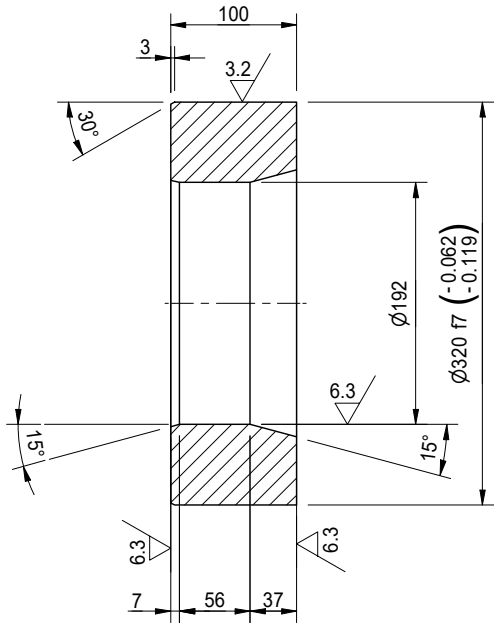
SECTION AT S1-S1 SCALE 1 : 6
